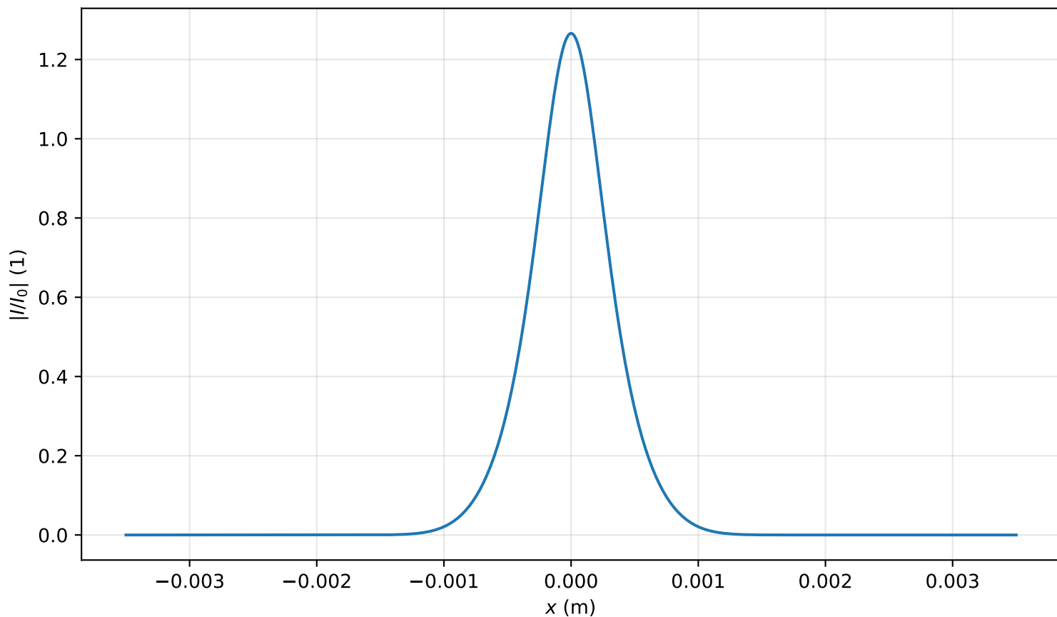
Intensity profile I(x, y = 0, z = 0.637m)/I_0 , P_{in}=1.0P_{cr} , artificial time
